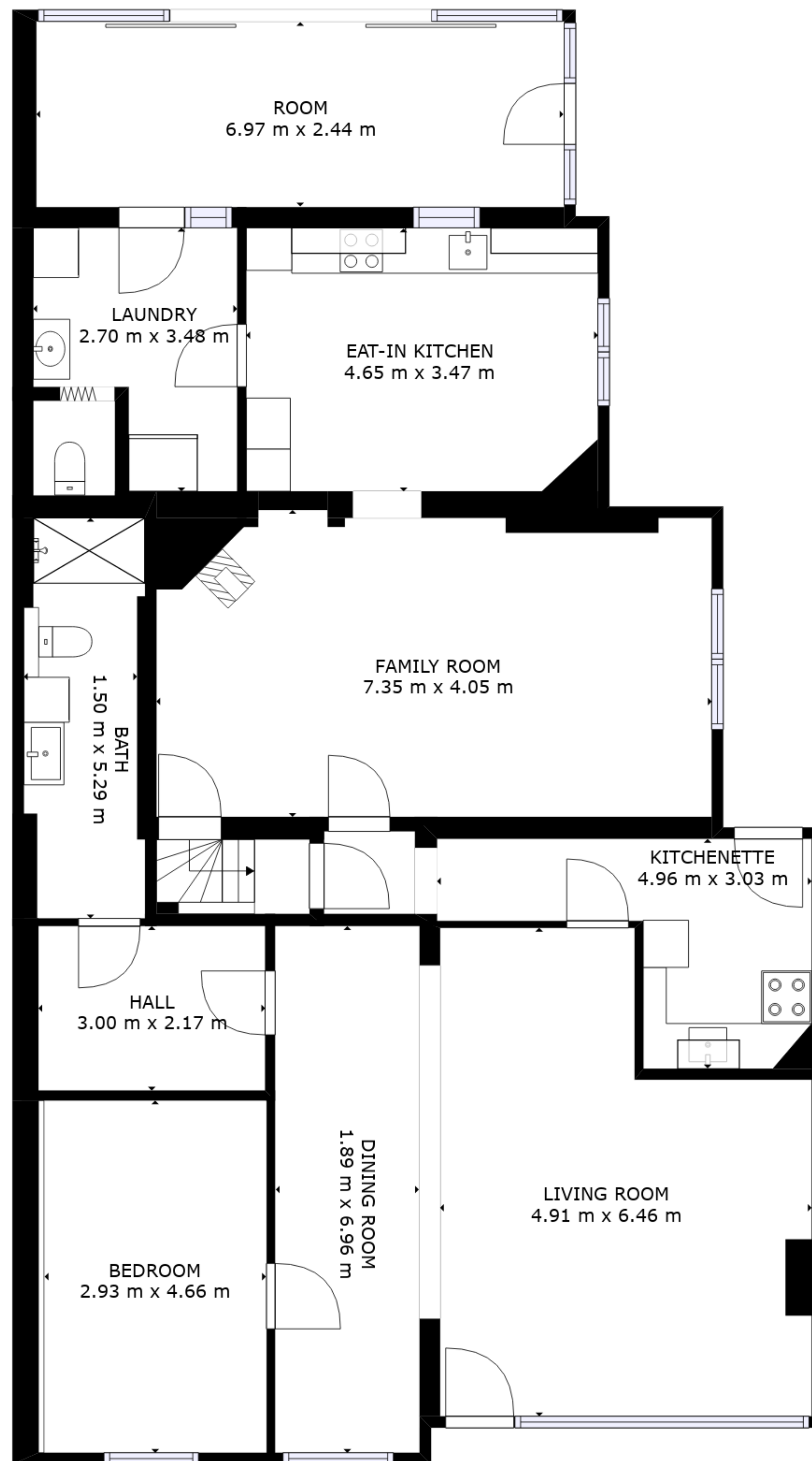
FLOOR 1
