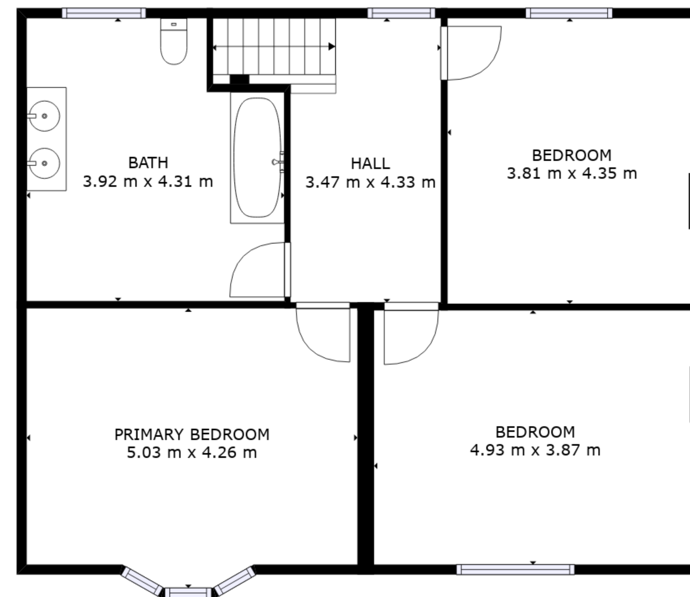
FLOOR 2
