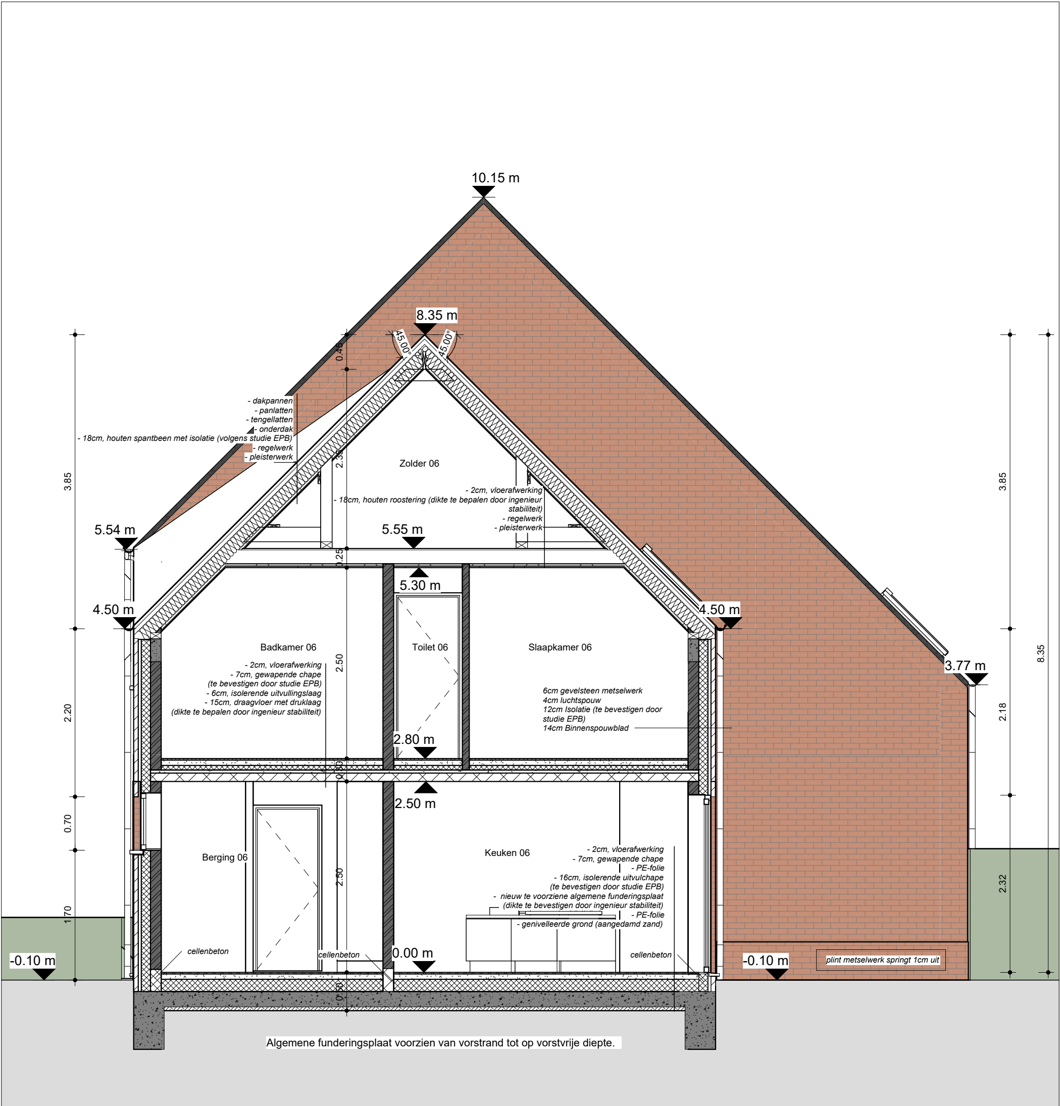
Snede C-C' - Lot 5
