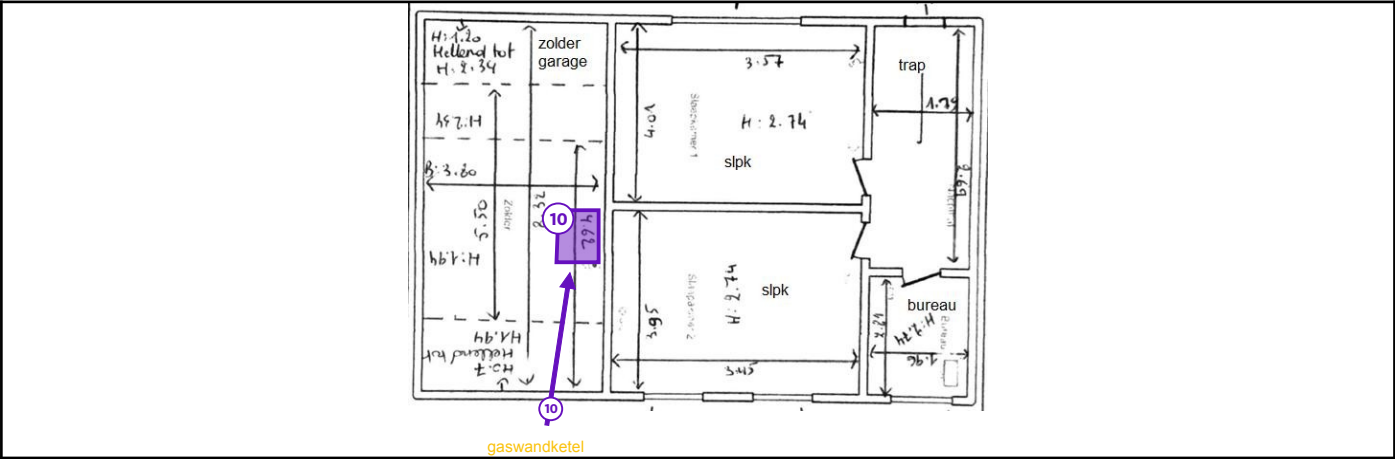
Legende van plan 1.9: Plan woning V+1
