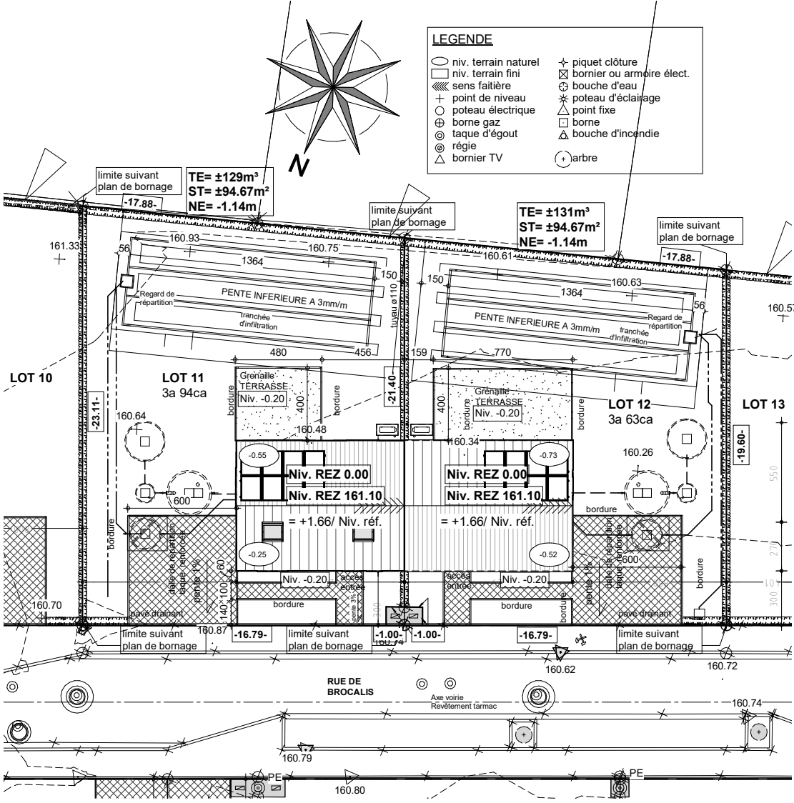
IMPLANTATION
