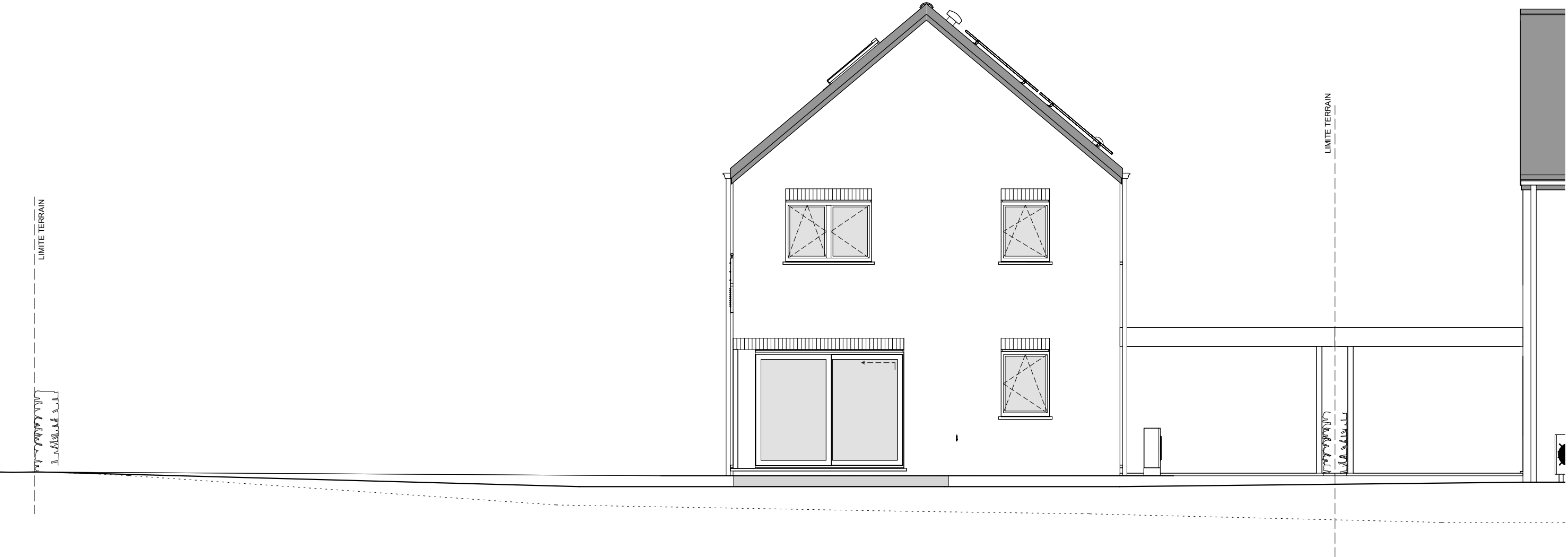
PIGNON ARRIERE
