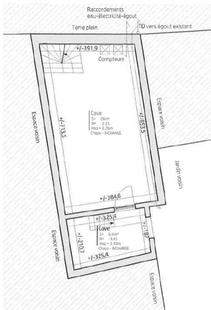
Plan caves
